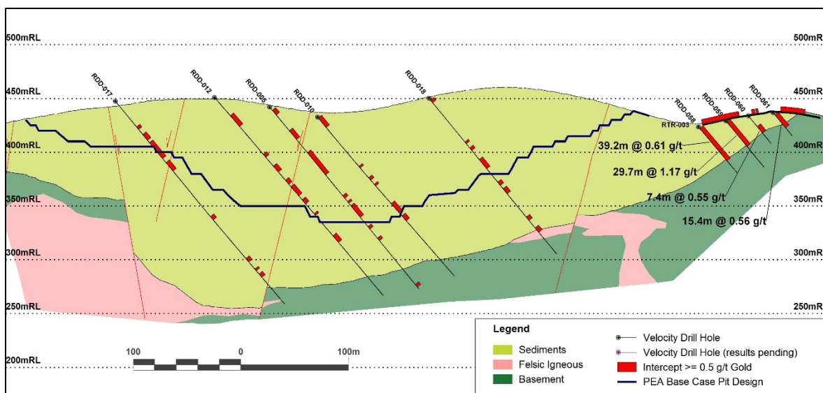
Figure 1: Cross-section showing drill intersections testing Trench RTR-003 at depth.
