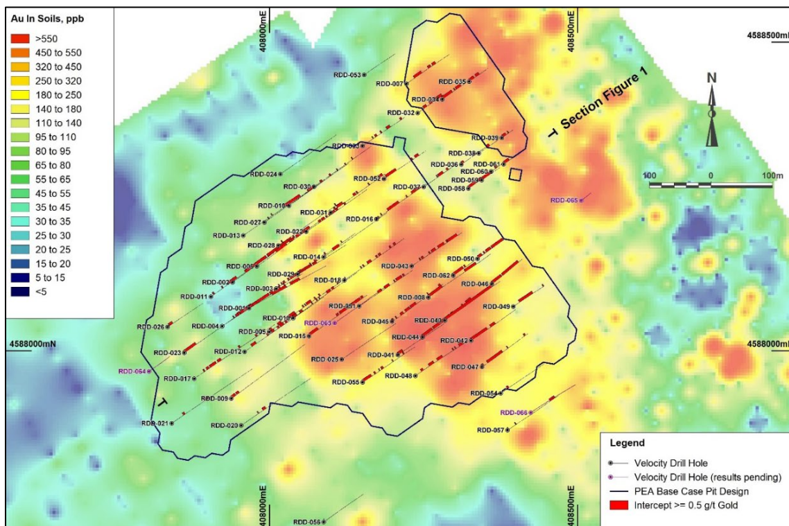
Figure 2: Map showing results for all Velocity drill holes and locations of drill holes for which results are pending. Gridded background shows gold-in-soil anomalies.
